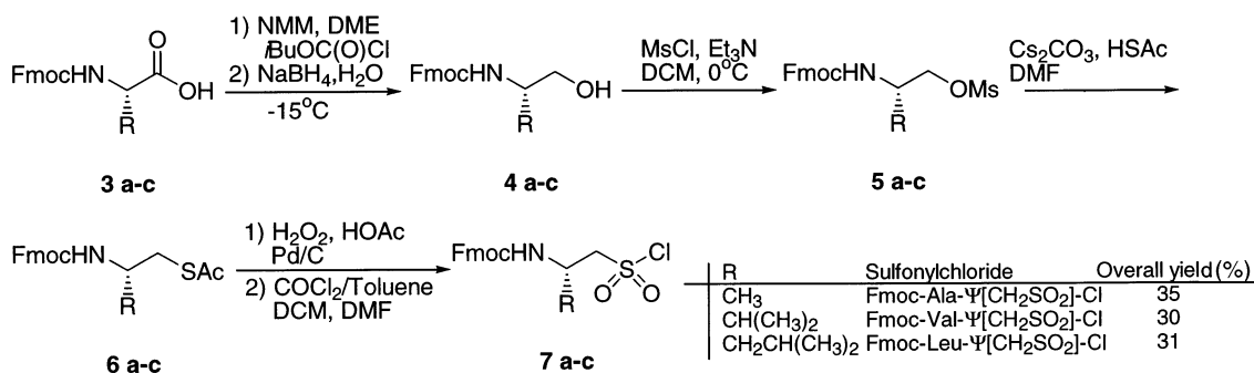
Scheme 1. Synthesis of the required Fmoc-protected β-aminoethanesulfonylchlorides 6
